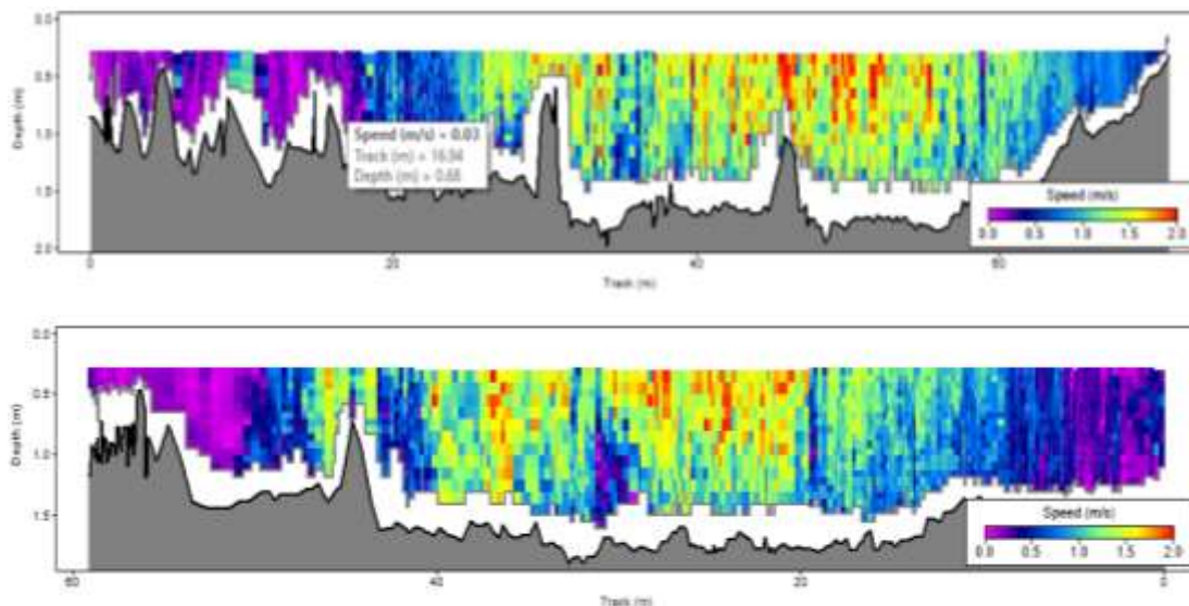
Figure 3. Cross section of the Saddang River upstream
