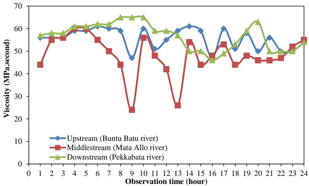
Figure 7. Viscosity at the Saddang River observation site
