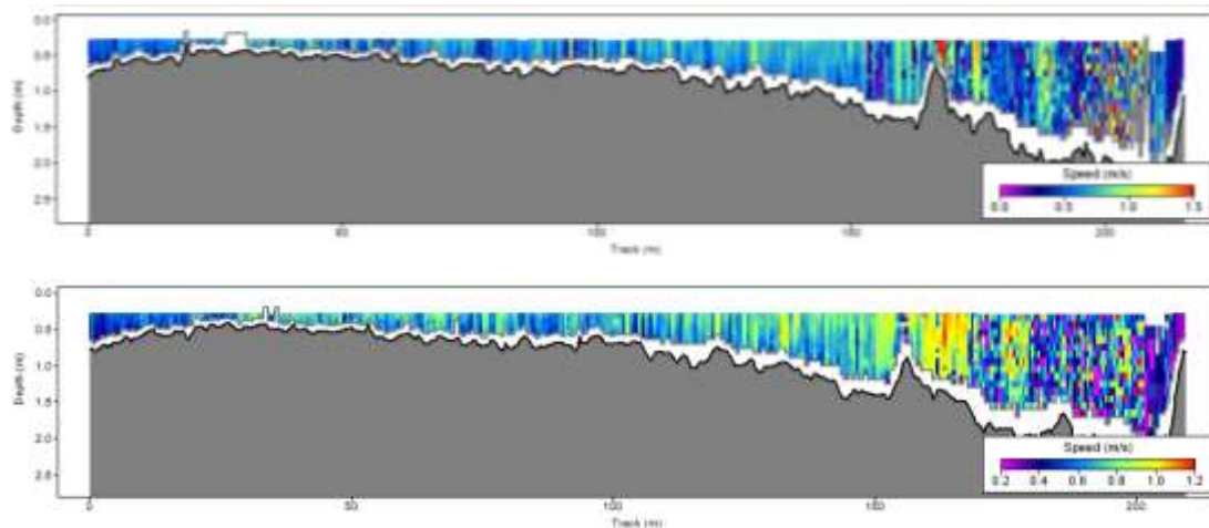
Figure 5. Cross section of the Saddang River downstream
